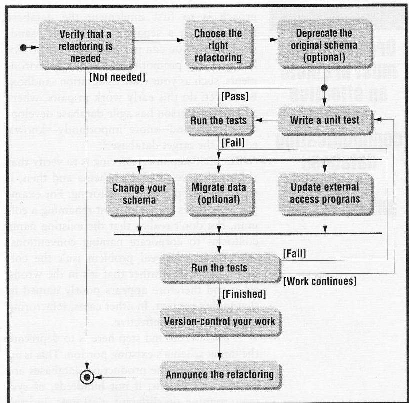
Figure 2. Database refactoring. Developers evolve the database schema in their own sandboxes before sharing the change with their teammates.
