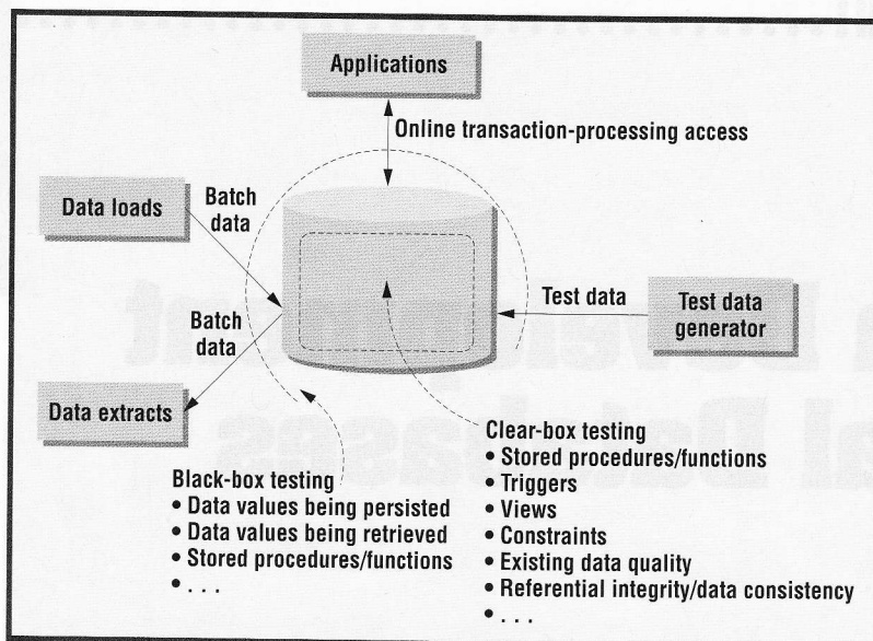
Figure 1. Testing a relational database. Developers must test the database both internally and at its interface—the equivalent of clear-box testing and black-box testing, respectively.
